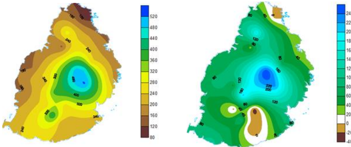
Fig. 1: (a) Observed rainfall (b) rainfall anomaly (mm)
