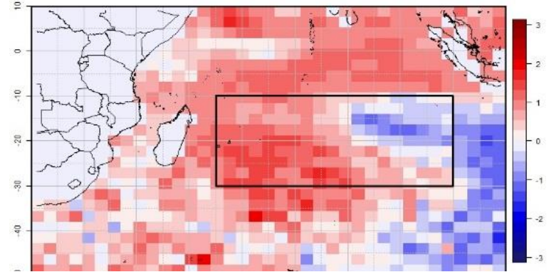
Figure 15: JFM sea surface temperature anomaly chart
