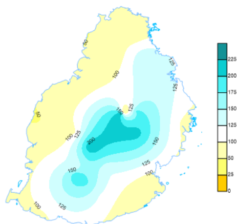
Observed Rainfall(mm)
