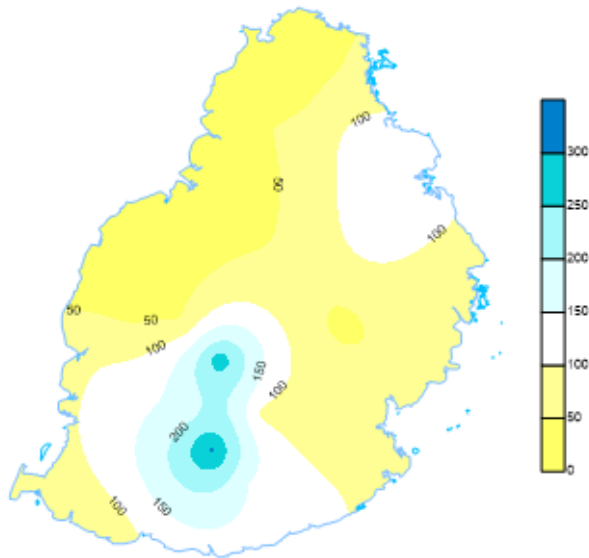
Observed Rainfall(mm)
